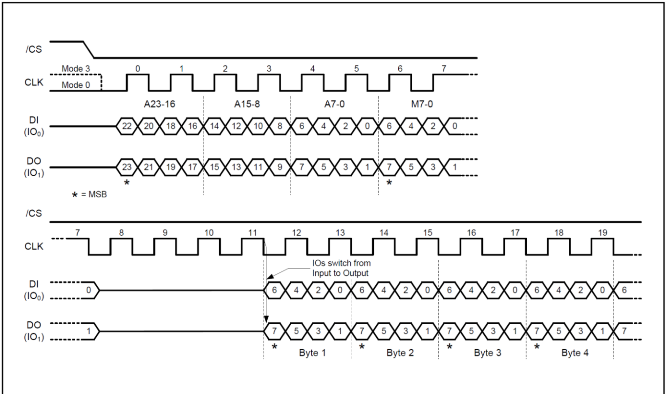
Figure 12b. DTR Fast Read Dual I/O (Previous instruction set M5-4=10, SPI Mode only)
